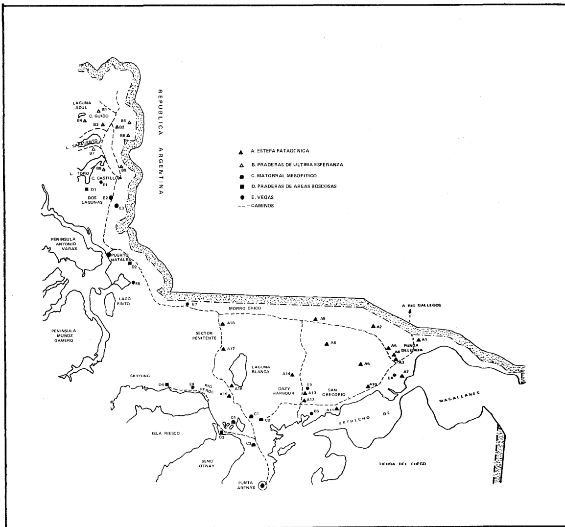
FIGURE 1. Sketch showing the approximate location of the sampling sites in Continental Magallanes.
